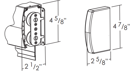
Mounting Bracket and End Cap Dimensions
